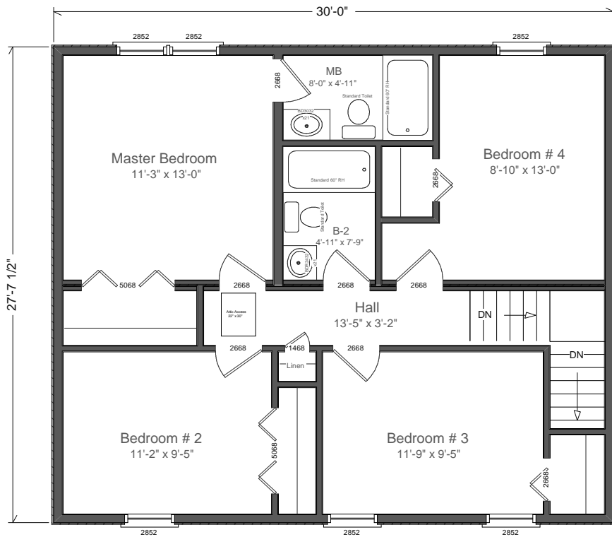
CMH-356 Second Floor 2830 Two Story Living Area 780 sq ft
