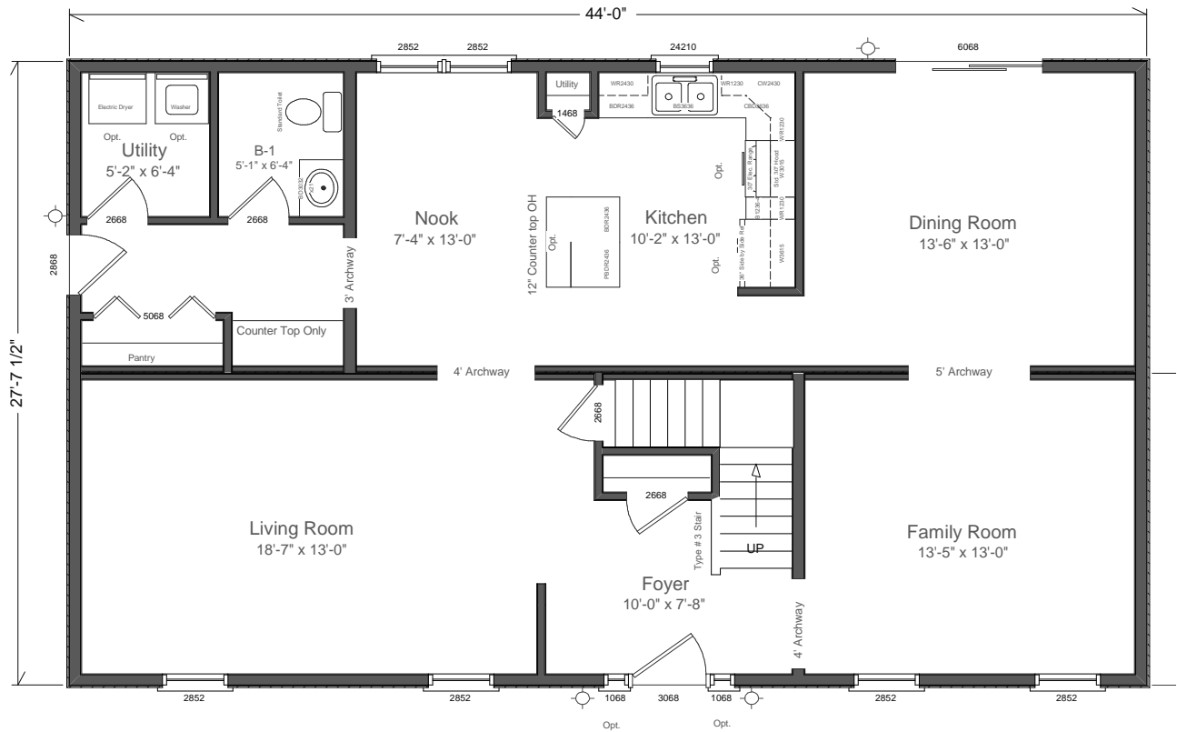
CMH-356 First Floor 2844 Two Story Living Area 1215 sq ft
