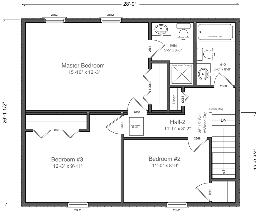
CMH-355 Second Floor 2628 Two Story Living Area 696 sq ft
