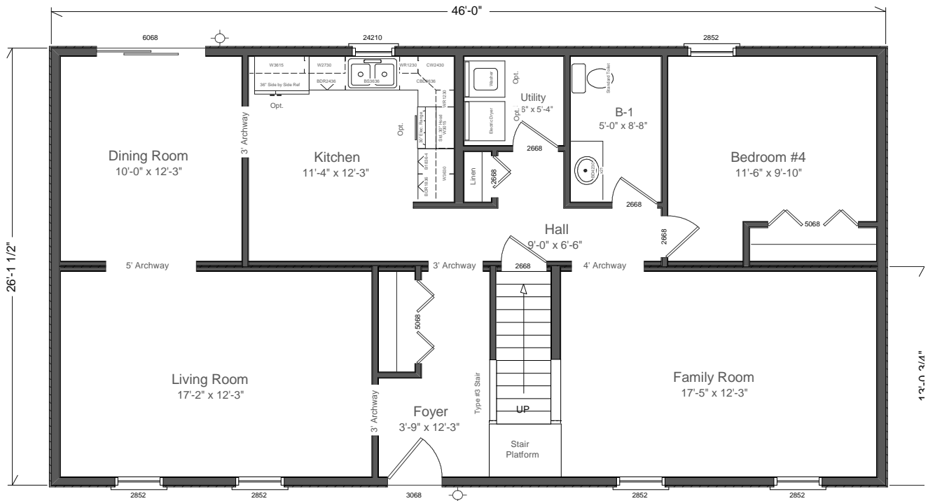
CMH-355 First Floor 2646 Two Story Living Area 1201 sq ft
