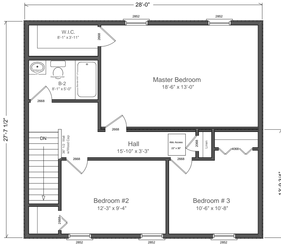
CMH-354 Second Floor 2828 Two Story Living Area 733 sq ft
