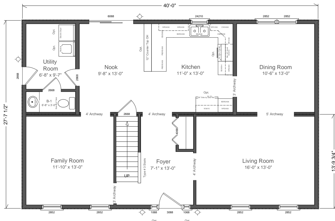
CMH-352 First Floor 2840 Two Story Living Area 1104 sq ft
