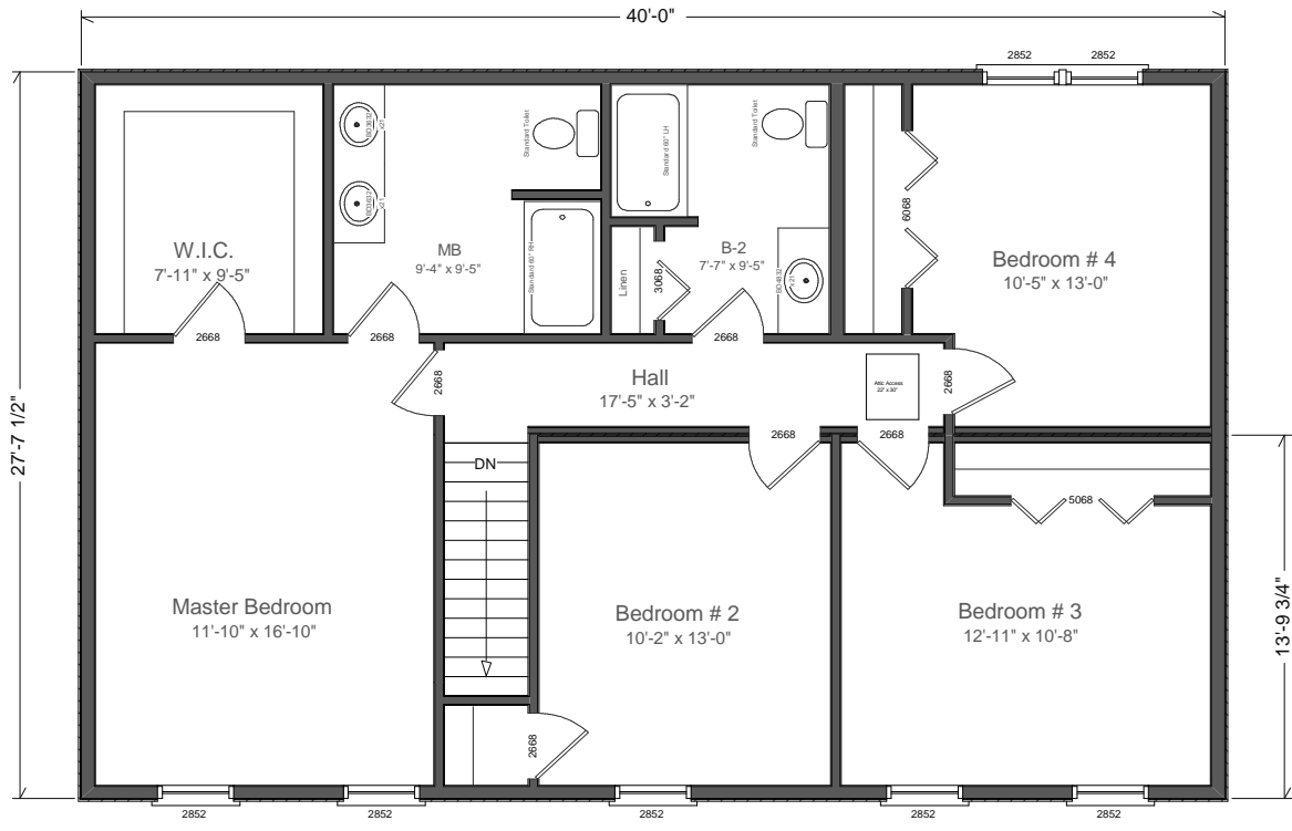
CMH-352 Second Floor 2840 Two Story Living Area 1071 sq ft
