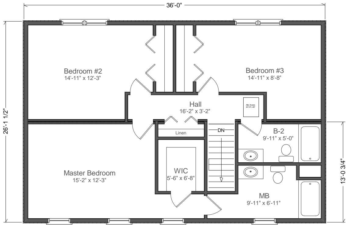
CMH-308 Second Floor 2636 Two Story Living Area 906 sq ft
