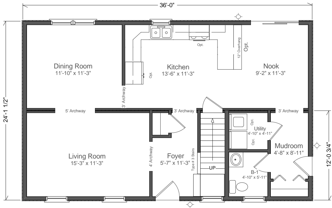
CMH-308 First Floor 2436 Two Story Living Area 868 sq ft
