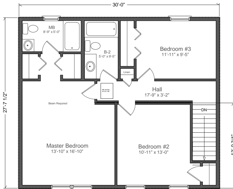
CMH-305 Second Floor 2830 Two Story Living Area 788 sq ft
