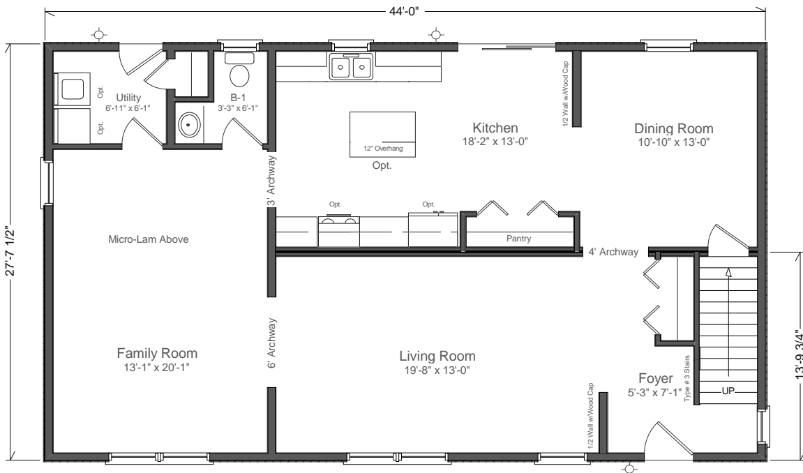
CMH-305 First Floor 2844 Two Story Living Area 1215 sq ft
