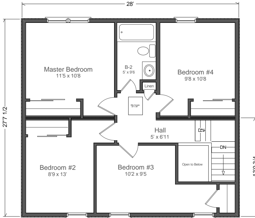
CMH-300 Second Floor 2828 Two Story Living Area 700 sq ft
