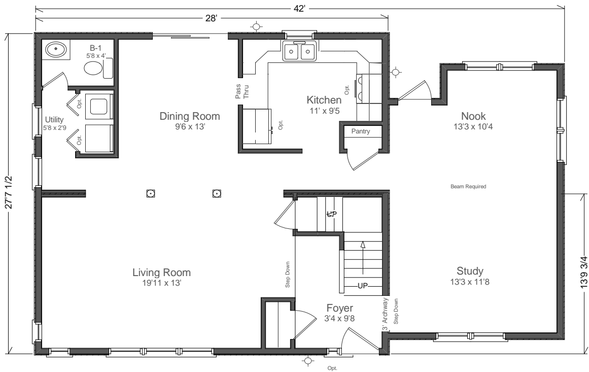
CMH-300 First Floor 2842 Two Story Living Area 1089 sq ft
