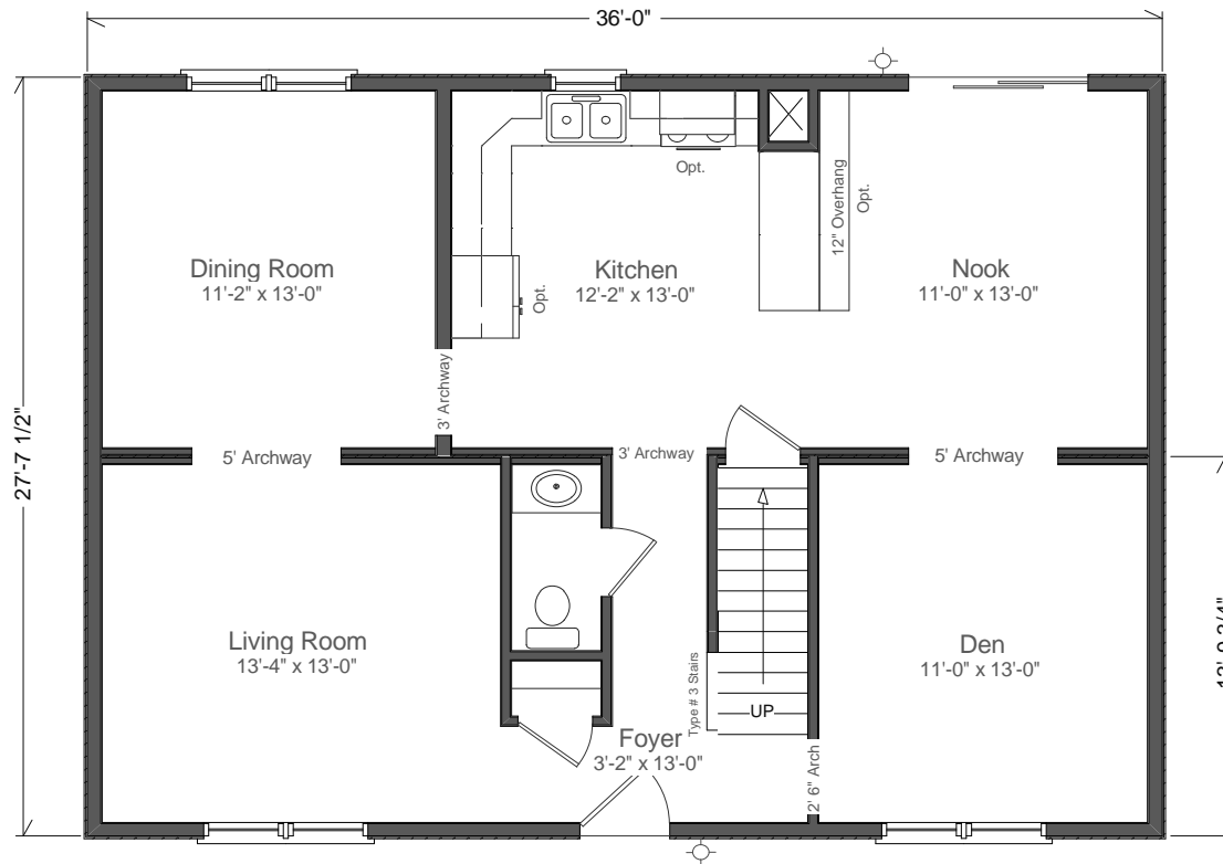
CMH-307 First Floor 2836 Two Story Living Area
