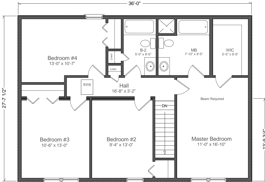
CMH-307 Second Floor 2836 Two Story Living Area 960 sq ft
