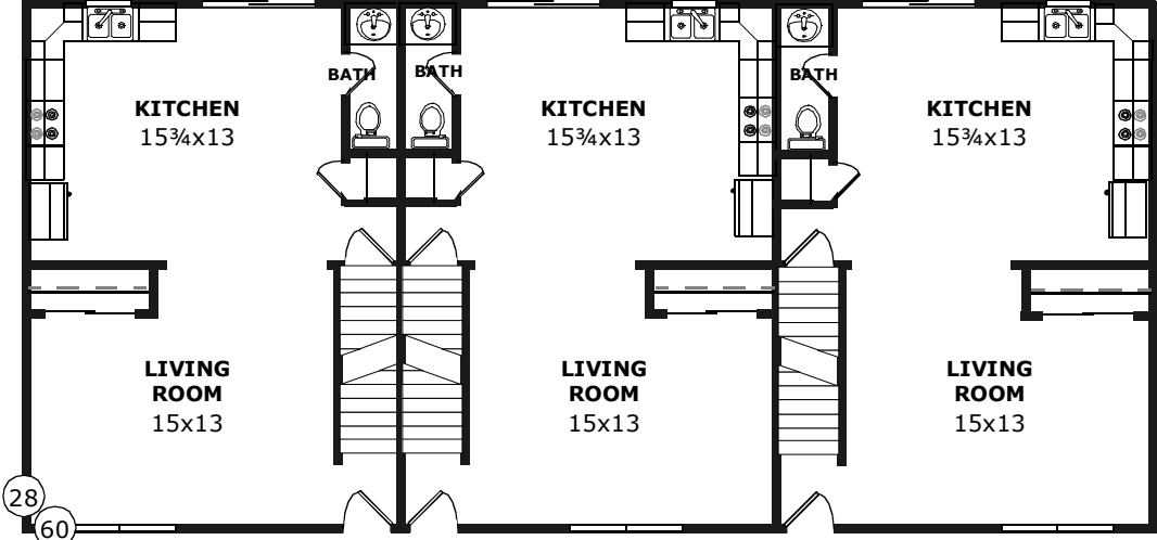
APT#1 1ST FLOOR
